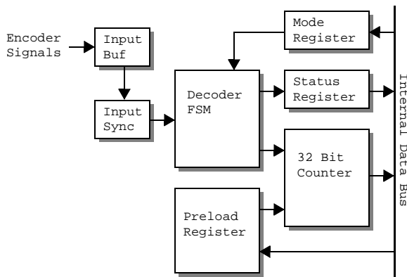
Figure 5: Encoder Interface Block Diagram
